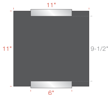
AS2L06-1111 6"w Bracket 11"h x 11"w Insert 9-1/2"h Display Area
