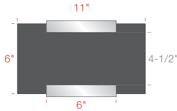
AS2L06-0611 6"w Bracket 6"h x 11"w Insert 4-1/2"h Display Area
