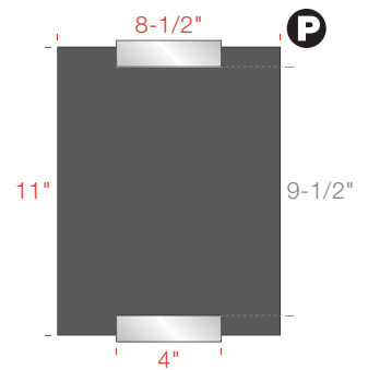
AS2L04-1185 4" w Bracket 11" h x 8-1/2" w Insert 9-1/2" h Display Area
