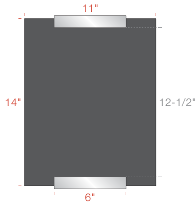
AS2L06-1411 6"w Bracket 14"h x 11"w Insert 12-1/2"h Display Area
