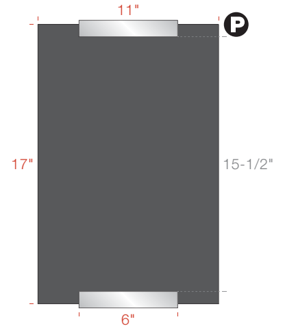
AS2L06-1711 6"w Bracket 17"h x 11"w Insert 15-1/2"h Display Area
