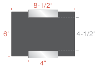
AS2L04-0685 4" w Bracket 6" h x 8-1/2" w Insert 4-1/2" h Display Area
