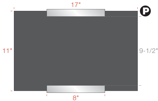
AS2L08-1117 8"w Bracket 11"h x 17"w Insert 9-1/2"h Display Area
