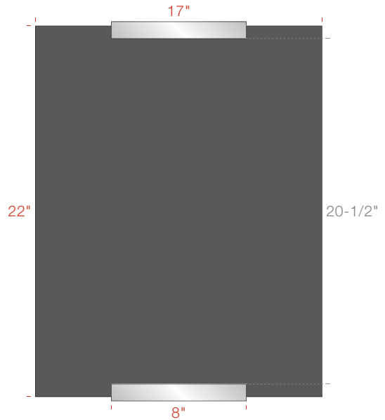
AS2L08-2217 8"w Bracket 22"h x 17"w Insert 20-1/2"h Display Area
