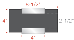
AS2L04-0485 4" w Bracket 4" h x 8-1/2" w Insert 2-1/2" h Display Area
