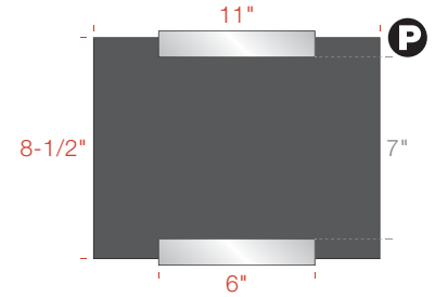
AS2L06-8511 6"w Bracket 8-1/2"h x 11"w Insert 7"h Display Area
