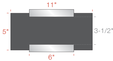
AS2L06-0511 6"w Bracket 5"h x 11"w Insert 3-1/2"h Display Area
