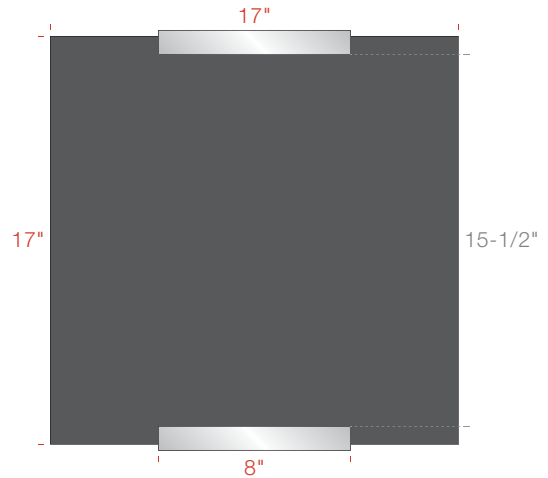
AS2L08-1717 8"w Bracket 17"h x 17"w Insert 15-1/2"h Display Area
