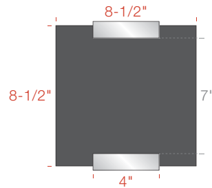
AS2L04-8585 4" w Bracket 8-1/2" h x 8-1/2" w Insert 7" h Display Area
