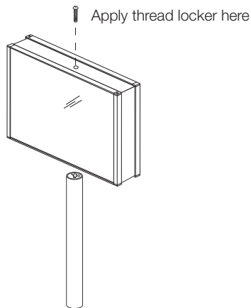
FS301.2 Two sided vertical
