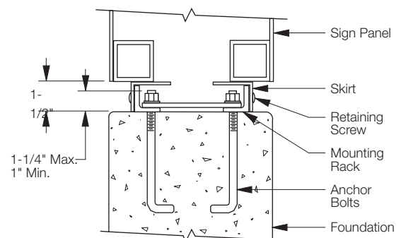
Anchor Detail
