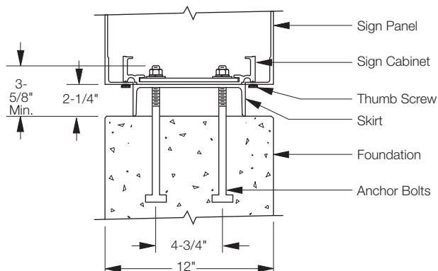
Anchor Detail
